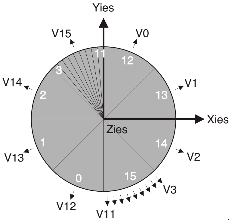
IES/ion in-plane
