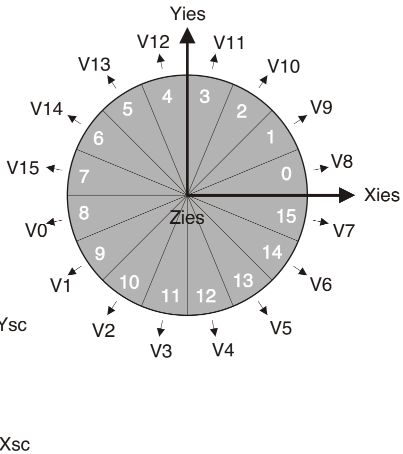
IES/electron in-plane
